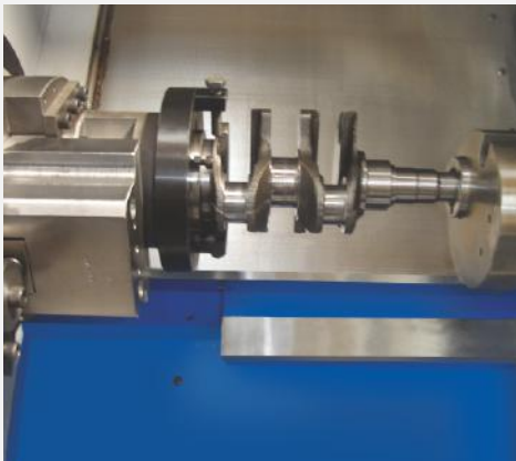
Eccentric collet system for Crank shaft pin turning
